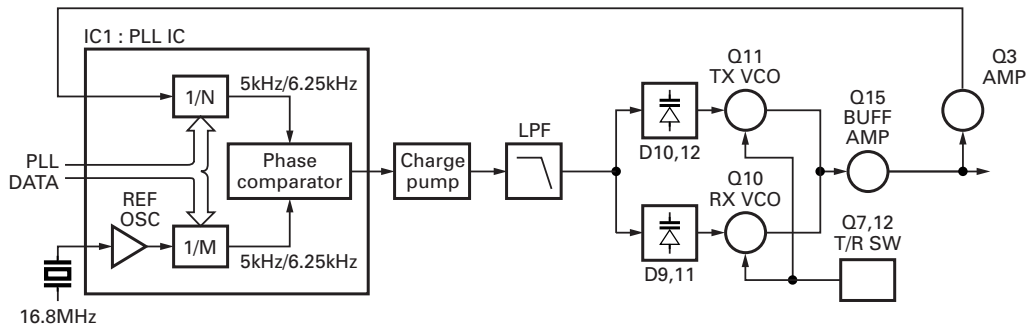
Fig. 6 PLL circuit
