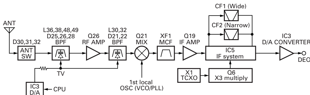
Fig. 2 Receiver system
