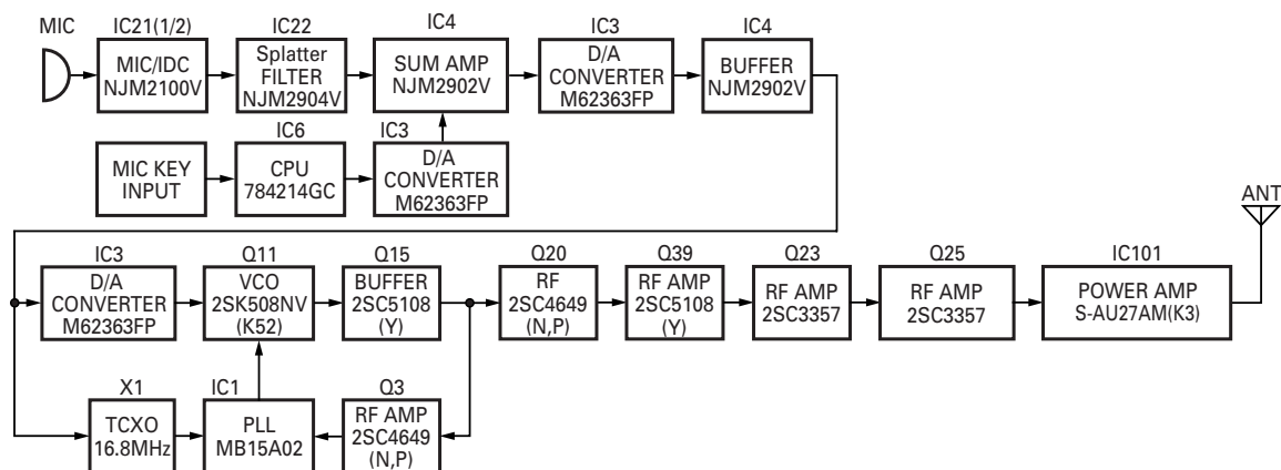
Fig. 8 Transmitter system
